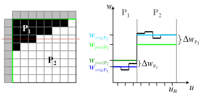
Figure 27: CPVs of block partitions: CPV prediction from adjacent samples of neighbouring blocks (left) and cross section of block (right), showing relation between different CPV types.
