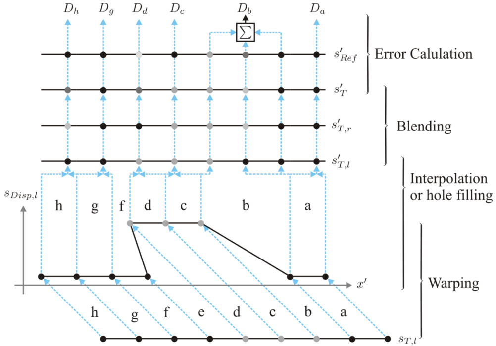
Figure 35: Example for the dependencies between input, intermediate and output signals of the rendering or error calculation step.
