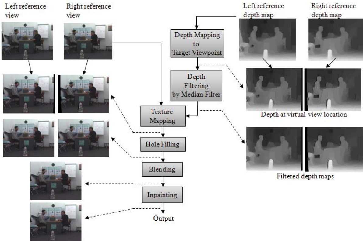
Figure 40: Flow diagram for VSRS general mode.
