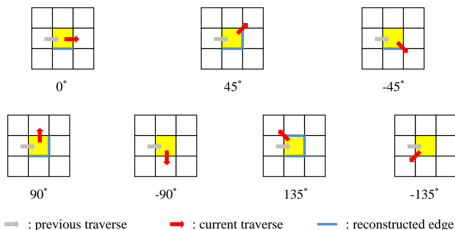
Figure 30: Reconstructed edge using the relationship between previous and current directions
