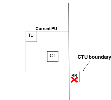
Figure 17: The BR temporal block below the lower CTU row is not considered
