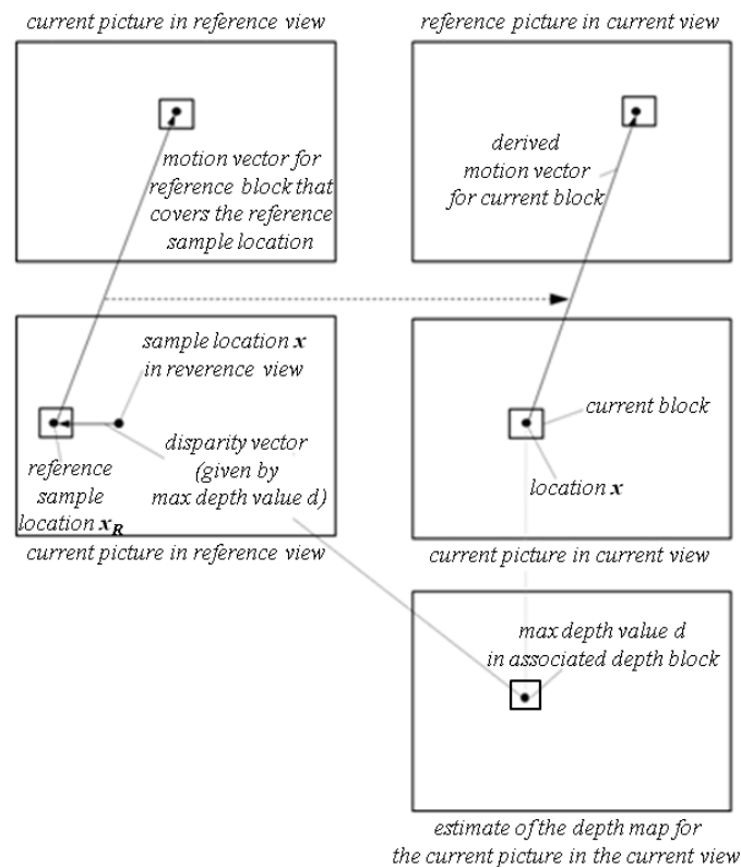
Figure 9: Basic principle of deriving motion parameters for a block in a current picture based on motion parameters in an already coded reference view and an estimate of the depth map for the current picture.
