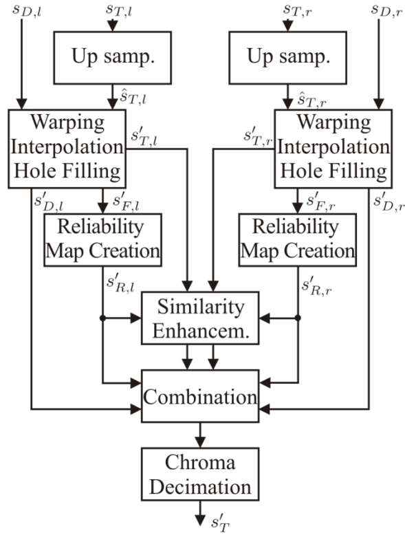
Figure 39: Processing steps of the view synthesis approach.
