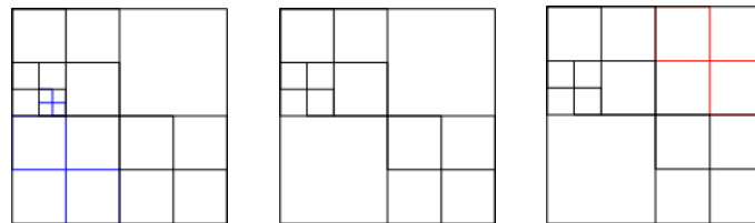
Figure 36: Example of a CTB QT partitioning for the texture (left), allowed collocated depth CTB QT partitioning (centre), and disallowed collocated depth CTB QT partitioning (right).
