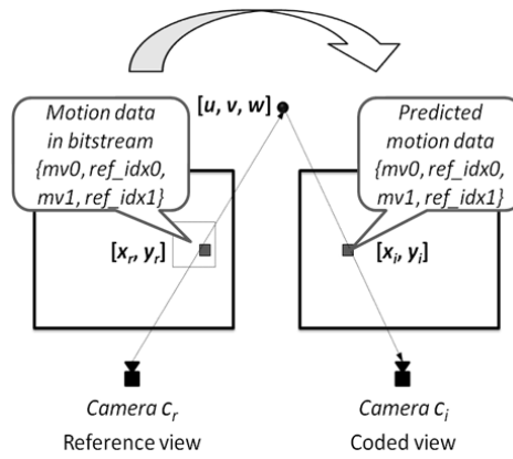
Figure 22: Independent derivation of motion information for each point of encoded CU from corresponding point in reference view.
