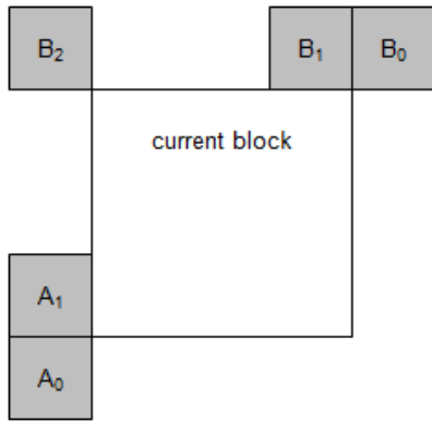
Figure 14: Location of spatial neighbour blocks
