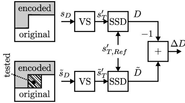
Figure 34: Definition of the SVDC related to the distorted depth data of the block B depicted by the hatched area in the bottom branch; VS denotes the view synthesis step and SSD stands for sum of squared differences.
