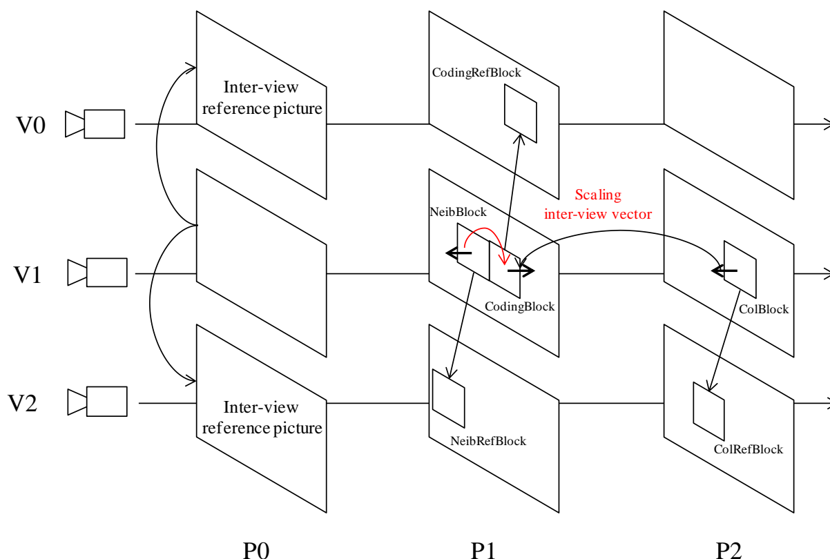
Figure 21: Inter-view motion vector scaling in AMVP and TMVP
