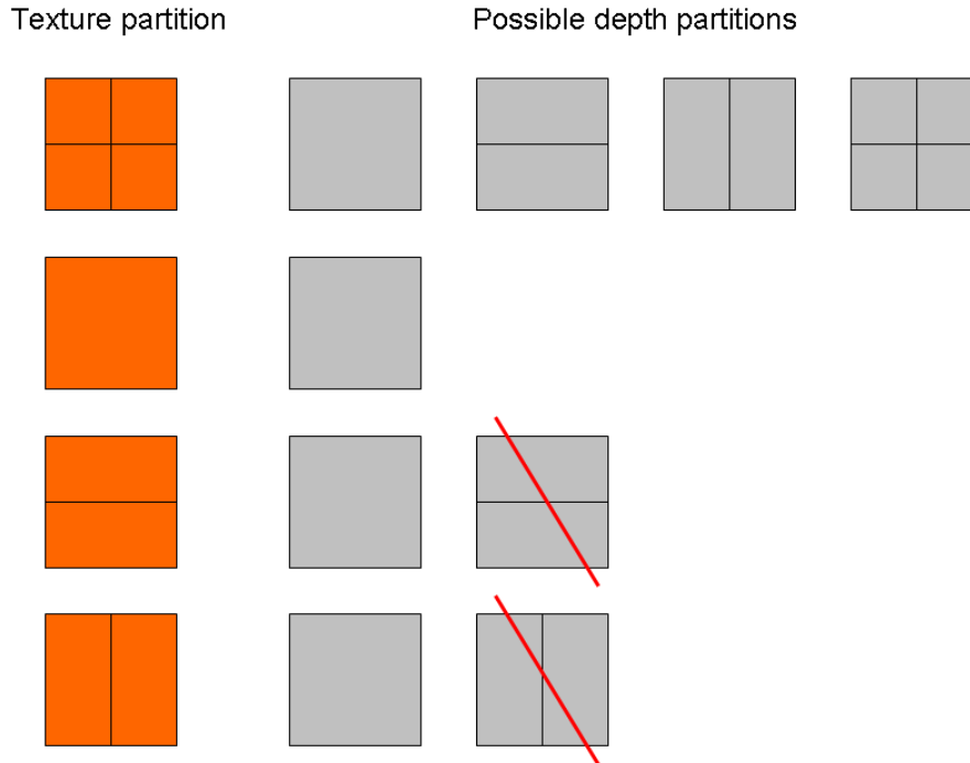
Figure 33: Texture partitions and corresponding possible depth partitions
