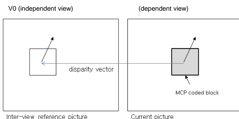
Figure 18: The inter-view predicted motion vector of a MCP coded block.
