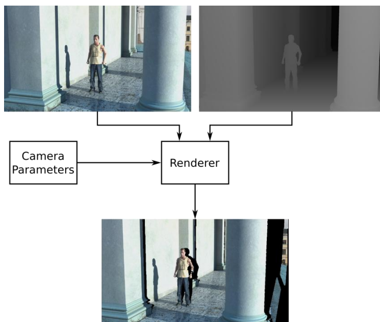
Figure 37: Rendering from a left camera position to a right camera position using depth maps.
